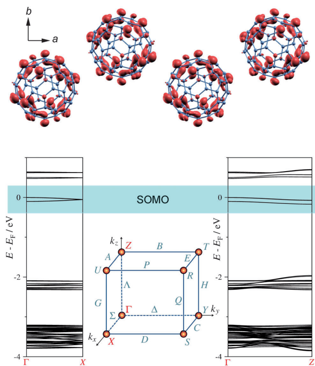
Figure 4. Spin density (top, isosurface at 0.014 \text{ e}^- \text{Å}^{-3} ) and sections of the band structure of \text{KC}_{60}(\text{THF})_5 \cdot 2\text{THF} (100 K), calculated at the B3LYP level. The band dispersion (majority spin) is represented along the \Gamma -X-line in the Brillouin zone, corresponding to the a axis in position space, and along the \Gamma -Z-line ( c axis). The partially filled bands at the Fermi level (0 eV) are highlighted (SOMO in the isolated anion). Details of the Brillouin zone are shown in the inset.
